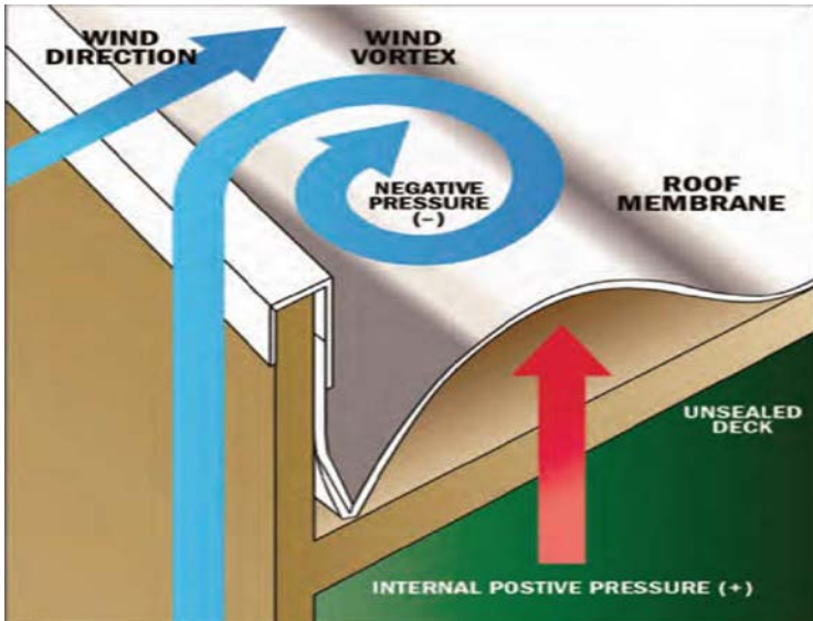
Mechanically attached Roofing System
